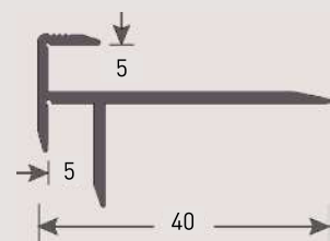
Double edge nosing, decoration series (aluminium)* Ref. 1605
